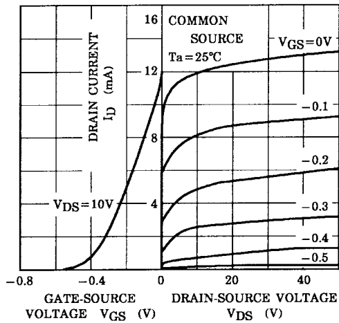
STATIC CHARACTERISTICS
